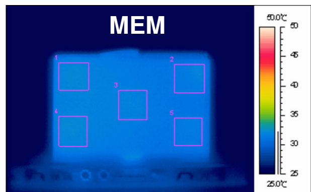
IR Temperature Measurement (5 point white, 30mins)
